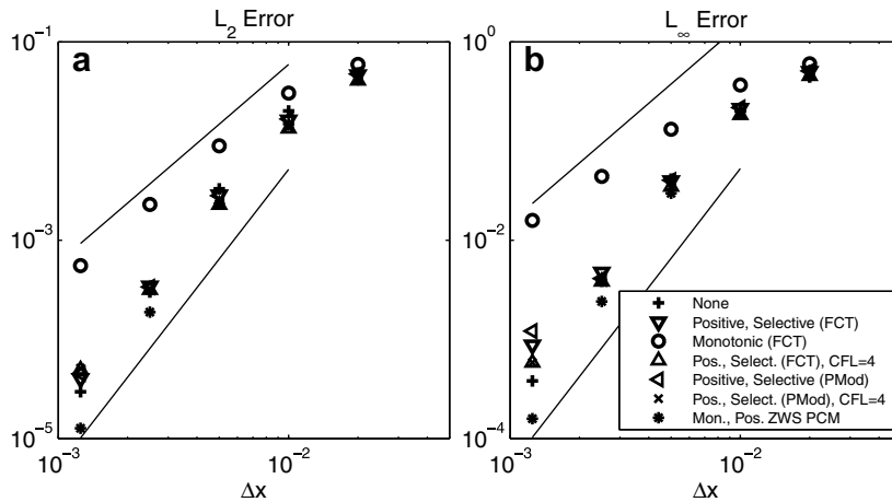
Fig. 14. Error, (a) E_2 and (b) E_\infty , as a function of numerical resolution. Solid lines show the slopes for second- and third-order convergence.
